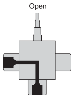
90° Three-Way Diverter Valve
