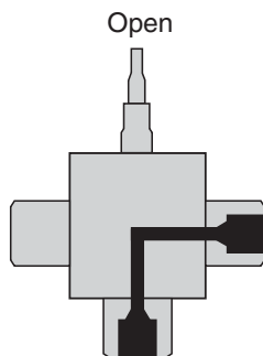
90° Three-Way Diverter Valve
