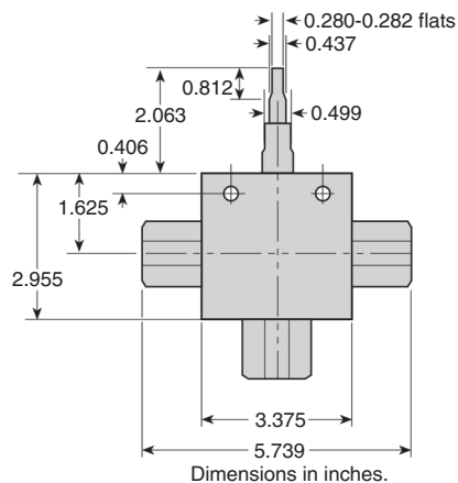
3-Way Ball Valve
