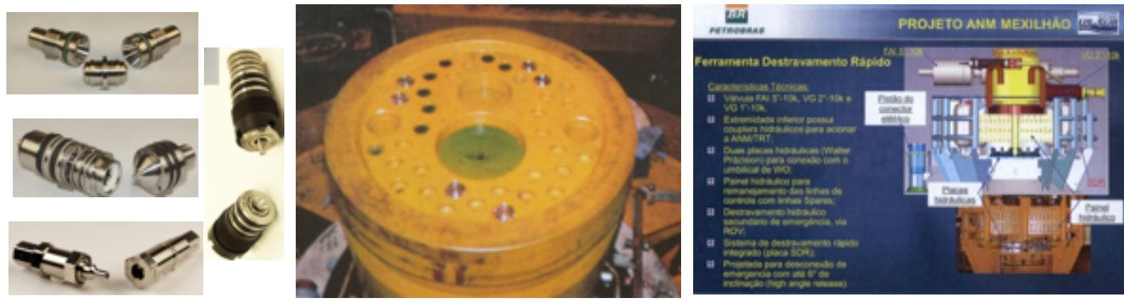
Coupling Elements with Metal, Polymer, or Resilient Seals, Buoy, FPSO and Gas Lift Connectors
